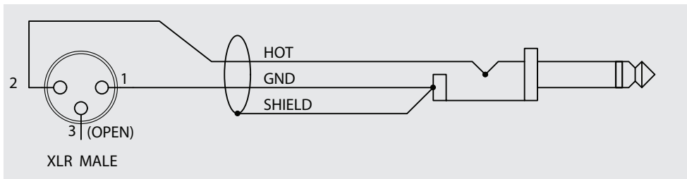
figure 1 - Unbalanced output cable termination
