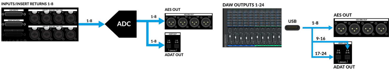
Normal mode - AES and ADAT Outputs fed from A-D converter
